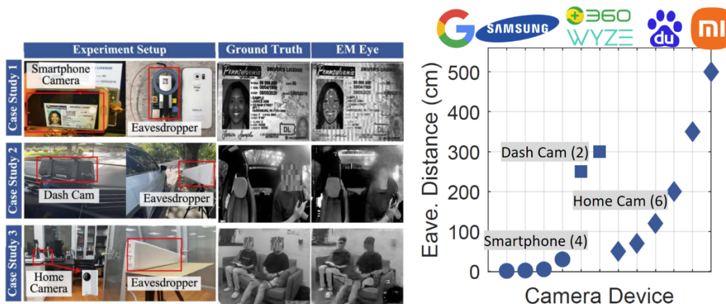
Figure 1: Example scenarios and susceptible devices of EM Eye attacks.
